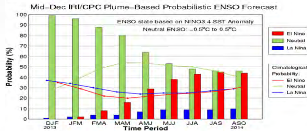
IRI Probabilistic ENSO Prediction for NINO3.4 Region
