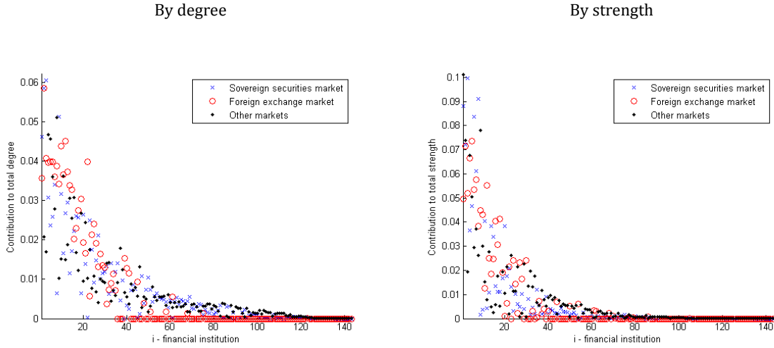
Figure 7. Positively correlated multiplexity. Participating FIs in each layer are ranked in decreasing order of degree (left) and strength (right) in the corresponding horizontal axis. High-degree and high-strength FIs in one layer tend to be the high-degree in the other two layers, which confirms the presence of positively correlated multiplexity.
